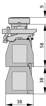
Push button with 2 rows of contacts
