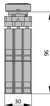
Push button with 2 rows of 3 contacts
